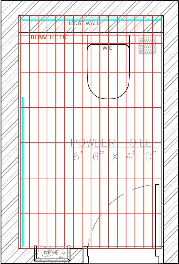
POWDER TOILET FLOORING PLAN
