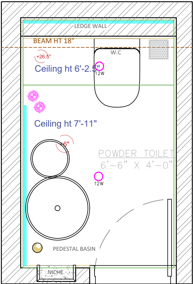
POWDER TOILET FALSE CEILING PLAN
