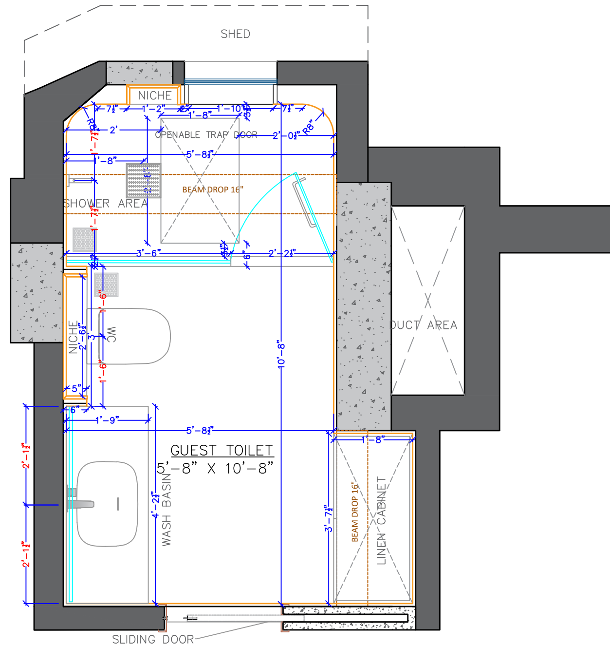
GUEST TOILET LAYOUT PLAN WITH MEASUREMENT
