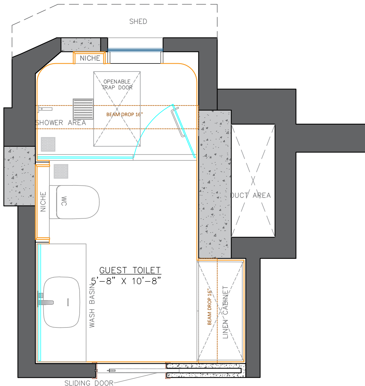
GUEST TOILET LAYOUT PLAN
