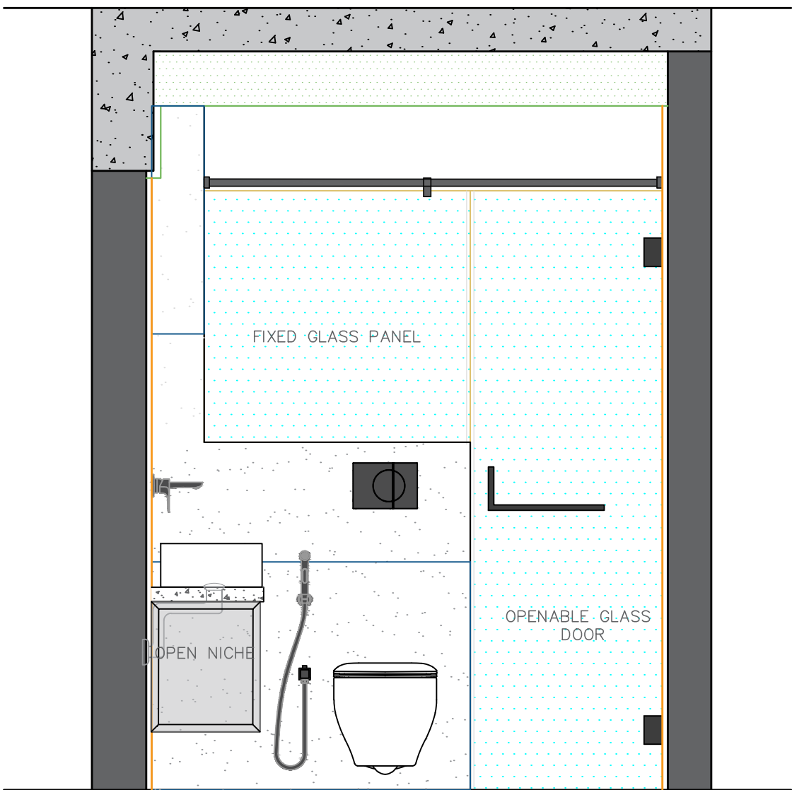
ELEVATION B-B' WITH GLASS DOOR
