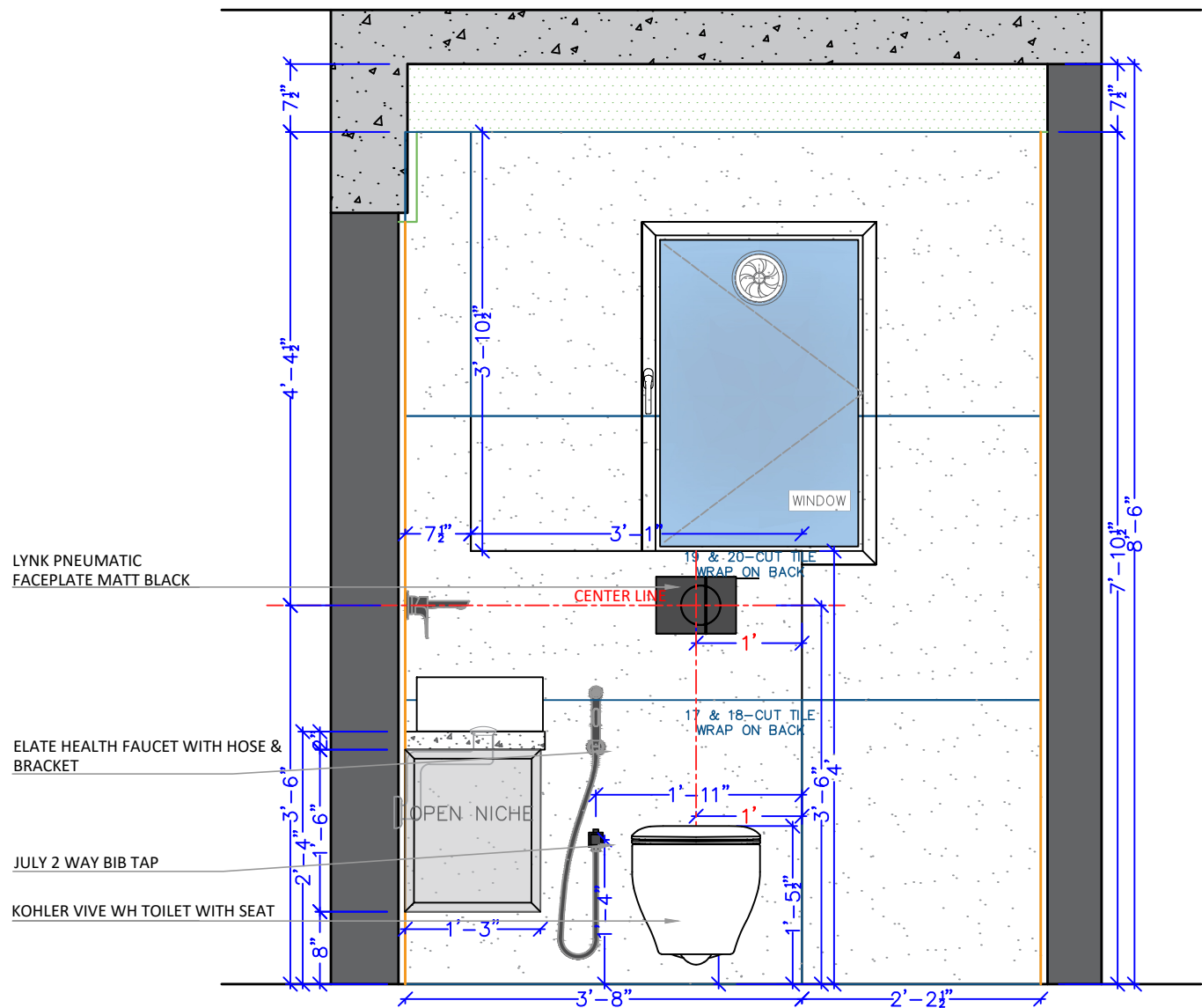
ELEVATION B-B' WITH WC AREA
