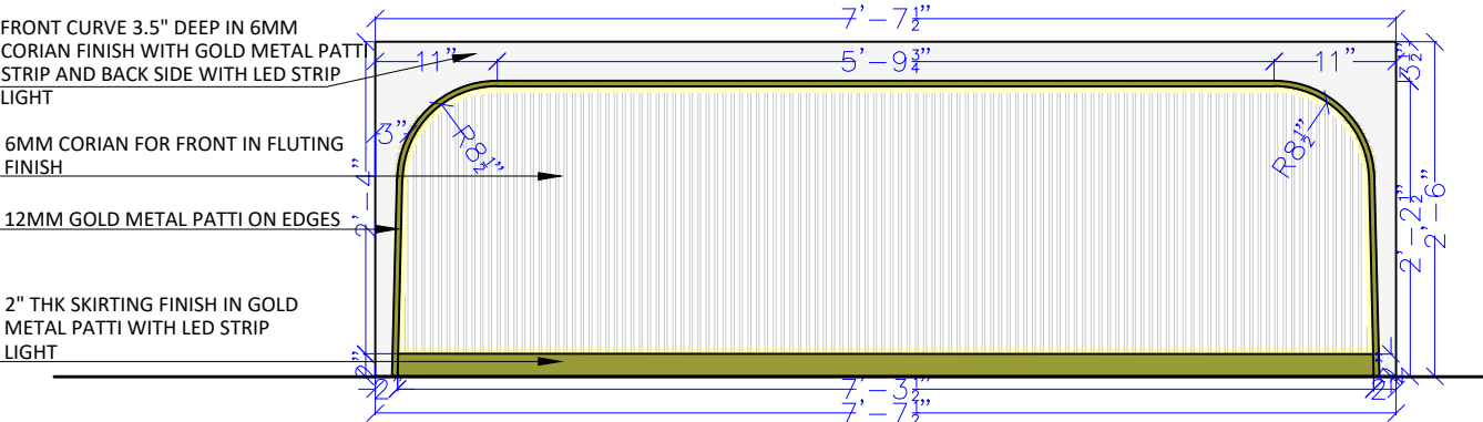
FRONT ELEVATION
