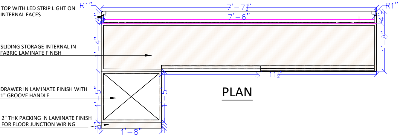
DISPLAY TABLE DETAIL DRAWING
