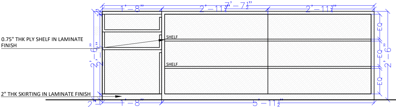
INTERNAL ELEVATION
