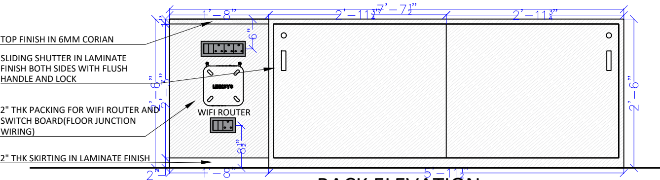
BACK ELEVATION
