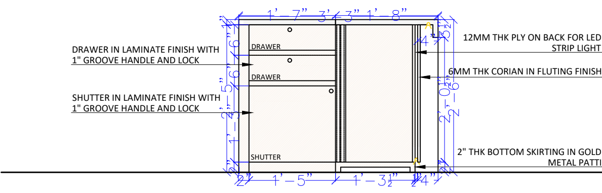
SECTION ELEVATION
