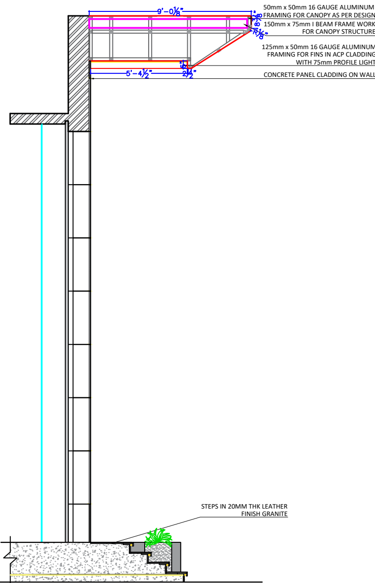
FACADE SIDE SECTION
