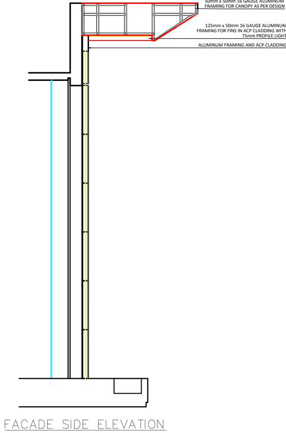
FACADE SIDE ELEVATION
