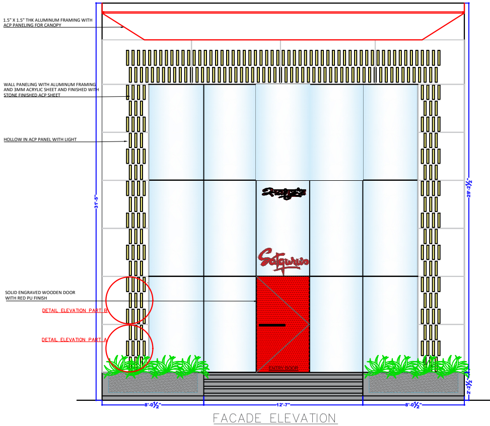
FACADE ELEVATION
