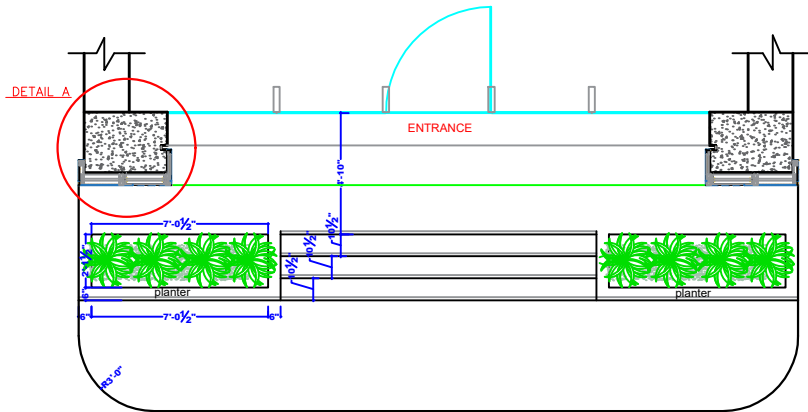
FACADE PLAN
